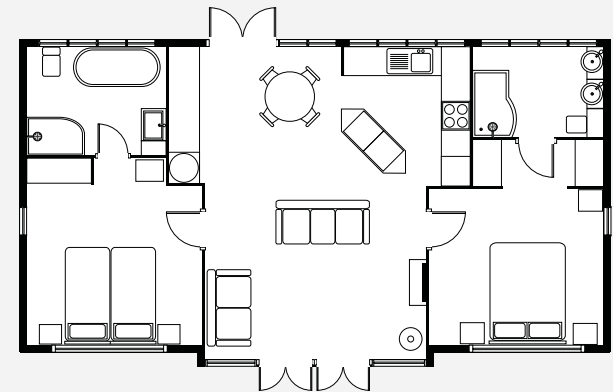
EXHIBITED MODEL: 40' x 22' (12.2m x 6.8m) Centre Living with double en suite
