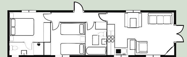
2 Bedroom, 2 Bathroom Lodge 45 x 12ft
